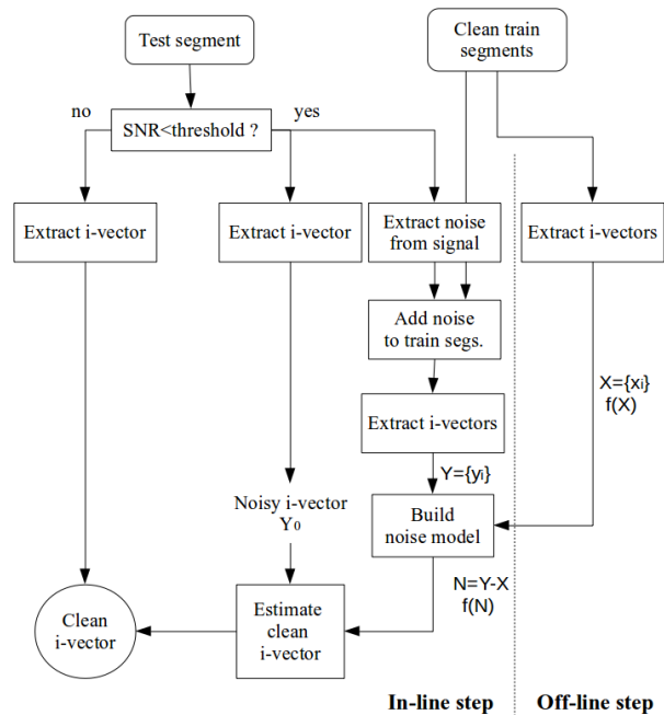
Figure 1: I-vector cleaning procedure using I-MAP.
