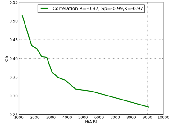
Figure 2: NHM behavioral curve for the pooled condition (all the comparison tests taken together).
